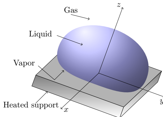
FIGURE 1: Leidenfrost effect.
