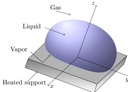
FIGURE 1: Leidenfrost effect.
