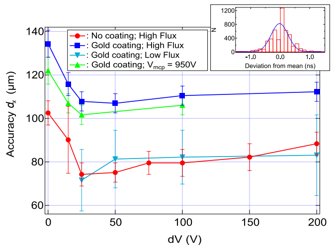
FIG. 8. Spatial accuracy d_x (as defined in Eq. 2) of the detectors as a function of dV and for different experimental configurations. Inset: Typical histogram of the centered distribution of D values measured in the experiment and from which \sigma_D is obtained.
