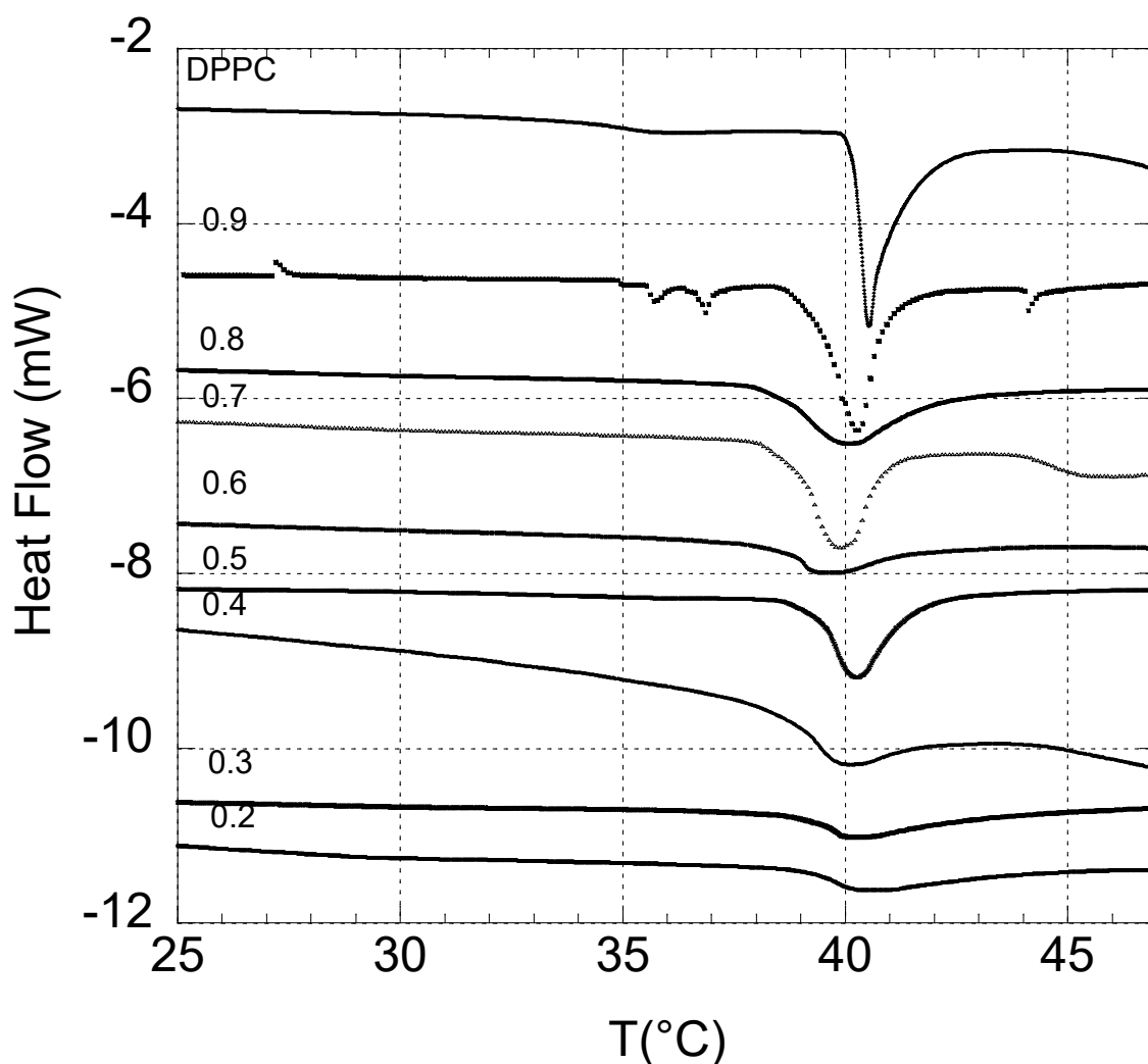
Figure S1: Thermograms obtained for vesicular suspensions of DPPC/PDMS-g-PEO
