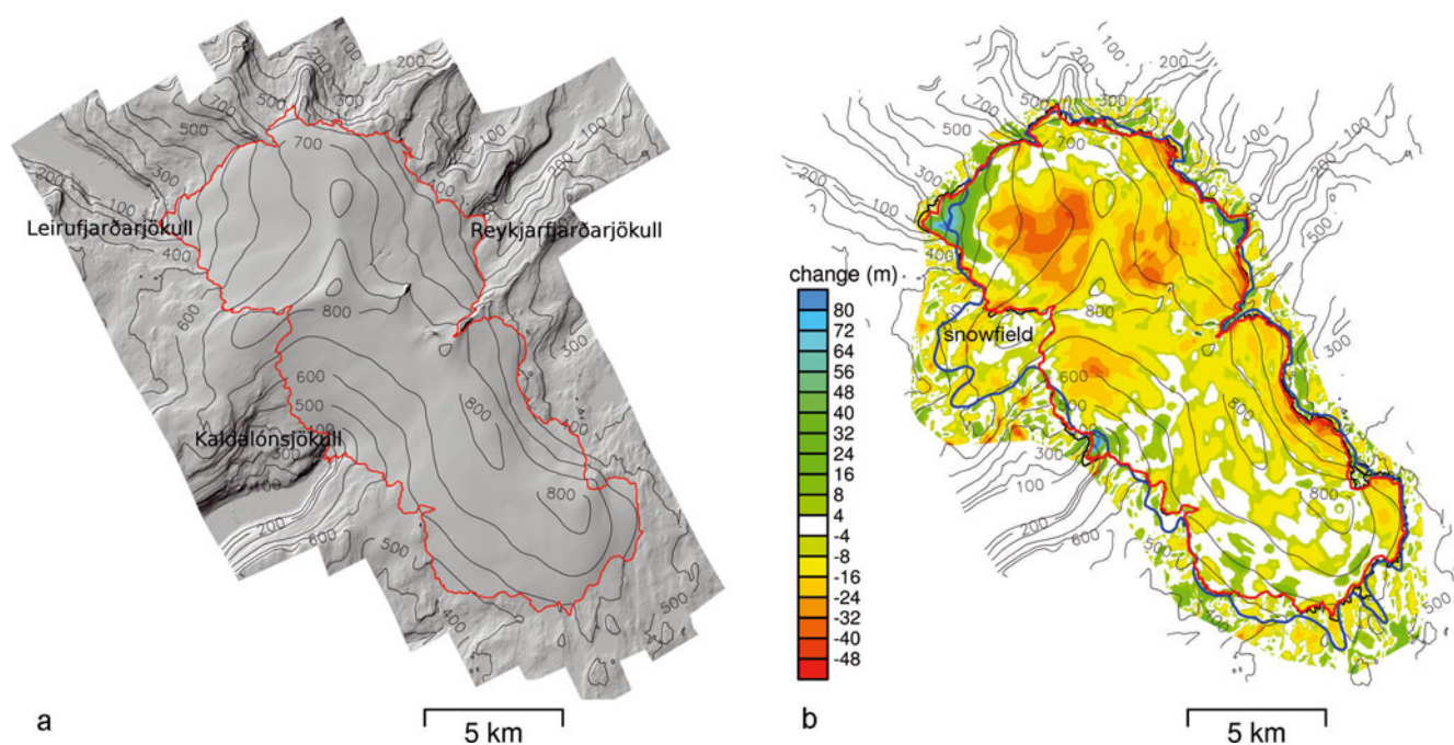
Fig. 3. (a) A hillshade of the 2011 lidar DEM of Drangajökull. (b) The difference in ice surface elevation between the ~1990 DMA map and the lidar DEM. Also shown is the outline of Drangajökull in ~1990 as drawn on the DMA map (blue curve), in 2004 as derived from orthorectified SPOT5 images (black curve) and as delineated from the lidar DEM (red curve, mostly overplotting the 2004 SPOT5 outline).
