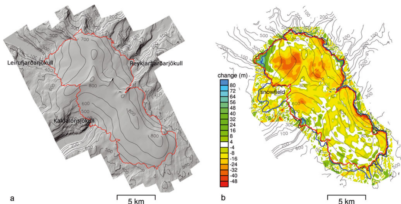
Fig. 3. (a) A hillshade of the 2011 lidar DEM of Drangajökull. (b) The difference in ice surface elevation between the \sim 1990 DMA map and the lidar DEM. Also shown is the outline of Drangajökull in \sim 1990 as drawn on the DMA map (blue curve), in 2004 as derived from orthorectified SPOT5 images (black curve) and as delineated from the lidar DEM (red curve, mostly overplotting the 2004 SPOT5 outline).
