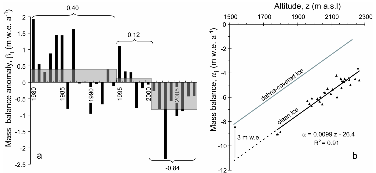
Figure 3: Output of the linear mass balance model (Lliboutry, 1974) applied to all mass balance measurements in the debris-free part of the ablation area of the Mer de Glace between September 1979 and September 2008 (29 hydrological years). (a) Annual mass balance anomaly ( \beta_t ). The grey boxes show the mass balance anomalies averaged over epochs I, II and III. (b) Relationship between the 1979-2008 average mass balances ( \alpha_i ) and altitude ( z ). The regression lines used on clean and debris-covered ice to compute the mass balance of the whole glacier tongue are also shown.
