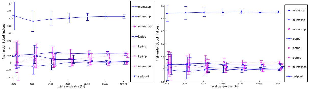
Figure 8. First-order SIs with error bars — 99% CI — for both Y_{\text{surf}} (left) and Y_{\text{depth}} (right).
