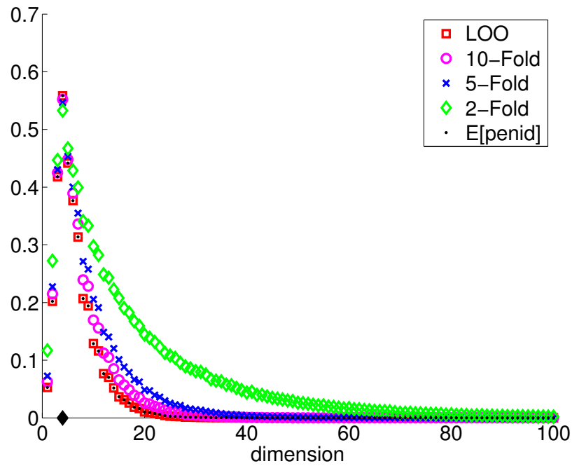
Figure 20: L-Regu, n = 100 . \bar{\Phi}(\text{SNR}_{\mathcal{C}}(m)) as a function of m .
