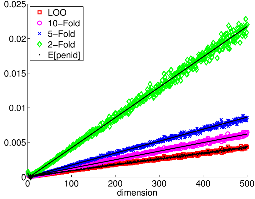
Figure 30: L-Regu, n = 500 . \text{Var}(\Delta_{\mathcal{C}_V}(m, m^*)) as a function of m . The black lines show the linear approximation n^{-2}[28(1 + \frac{0.06}{V-1}) + 2.1(1 + \frac{4.2}{V-1})(m - m^*)] for m > m^* = 7 .
