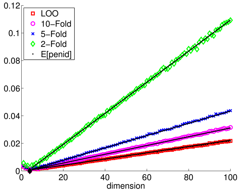
Figure 19: L-Regu, n = 100 . \text{Var}(\Delta_{\mathcal{C}}(m, m^*)) as a function of m . The black lines show the linear approximation n^{-2}[5.6(1 + \frac{1.1}{V-1}) + 2.2(1 + \frac{4.2}{V-1})(m - m^*)] for m > m^* = 4 .
