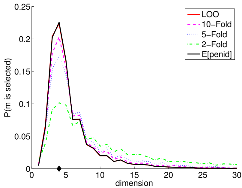
Figure 21: L-Regu, n = 100 . \mathbb{P}(\hat{m}(\mathcal{C}) = m) as a function of m .
