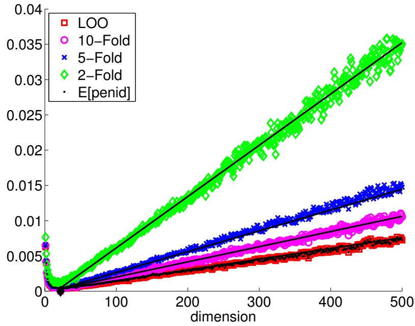
Figure 25: S-Regu, n = 500 . \text{Var}(\Delta_{\mathcal{C}_V}(m, m^*)) as a function of m . The black lines show the linear approximation n^{-2}[75(1 + \frac{0.52}{V-1}) + 3.8(1 + \frac{3.8}{V-1})(m - m^*)] for m > m^* = 22 .
