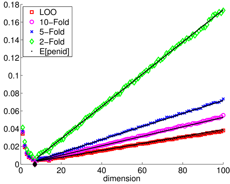
FIGURE 3. Illustration of the variance heuristic: \text{var}(\Delta_C(m, m^*)) as a function of m for five different C . Setting S -Regu, n = 100 . The black diamond shows m^* = 7 . The black lines show the linear approximation n^{-2}[29(1 + \frac{0.81}{V-1}) + 3.7(1 + \frac{3.8}{V-1})(m - m^*)] for m > m^* .
