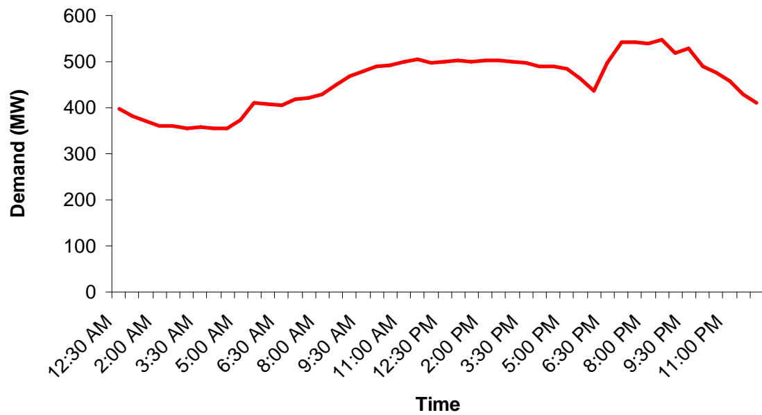
Figure 8 Typical daily load demand profile of Jamaica
