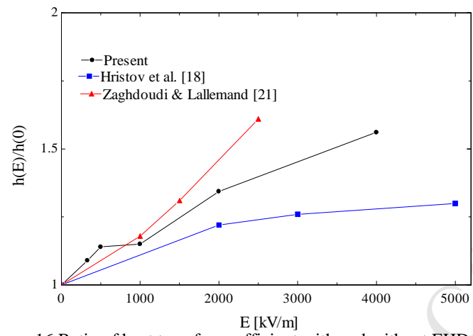
Figure 16 Ratio of heat transfer coefficient with and without EHD at 100 kW/m 2
