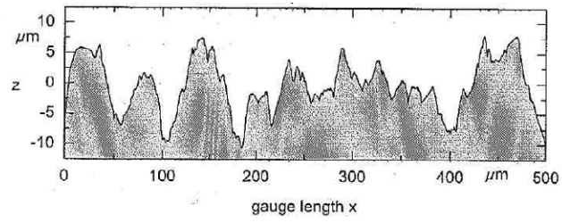
Figure 4 Profile of heating surface (enlargement z/x = 6.35 ), P_a = 3.5 \mu\text{m} .
