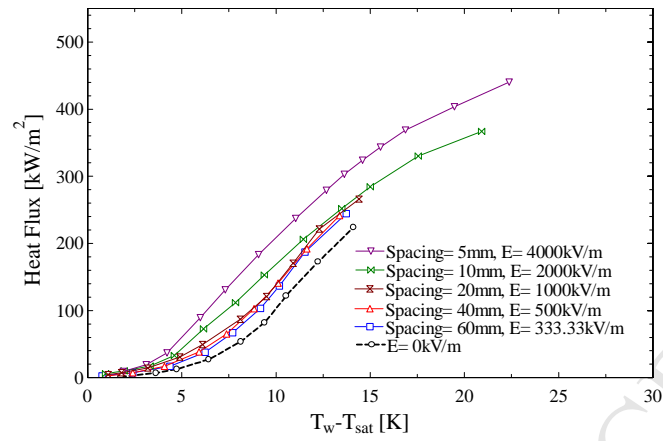
Figure 13 EHD results with variable electrode spacing voltage applied: zero and 20 kV for decreasing heat flux.
