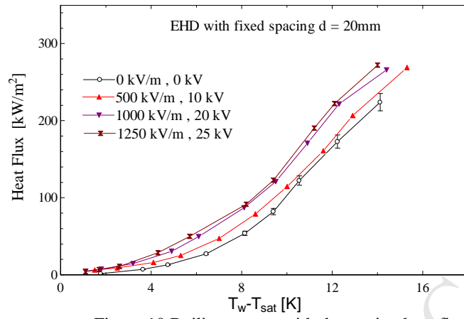
Figure 10 Boiling curves with decreasing heat flux.
