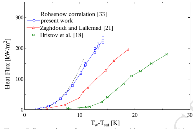
Figure 7 Comparison of present results with past work, without EHD.
