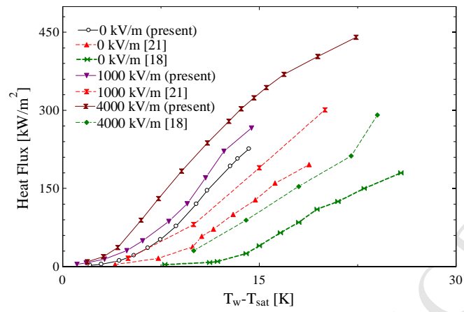
Figure 15 Effect of compound enhancement
