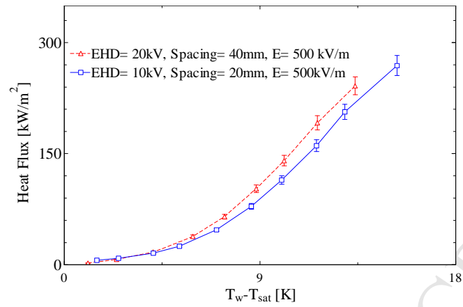
Figure 14 Comparison of same electric field at different electrode spacing.
