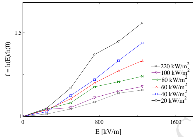
Figure 12 Heat transfer augmentation at fixed electrode spacing, 20 mm.
