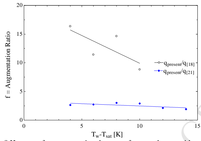
Figure 8 Heat transfer augmentation due to surface roughness, without EHD.
