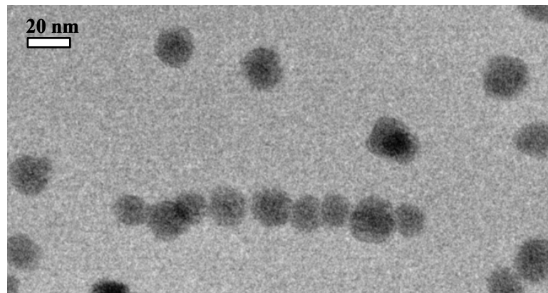
Figure 3. Cryo-TEM image of C_{chitosan}=0.01g/l / C_{SiNP}=10g/l solutions with C_{CH_3COOH} = 0.3 M and C_{CH_3COONa} = 0.2 M.
