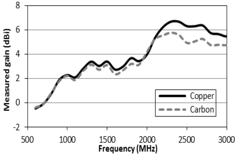
Figure 6. Maximum measured gains (from 600 MHz to 3 GHz) of the carbon-fiber monopole antenna (grey dashed line) and of the copper counterpart (black solid line).
