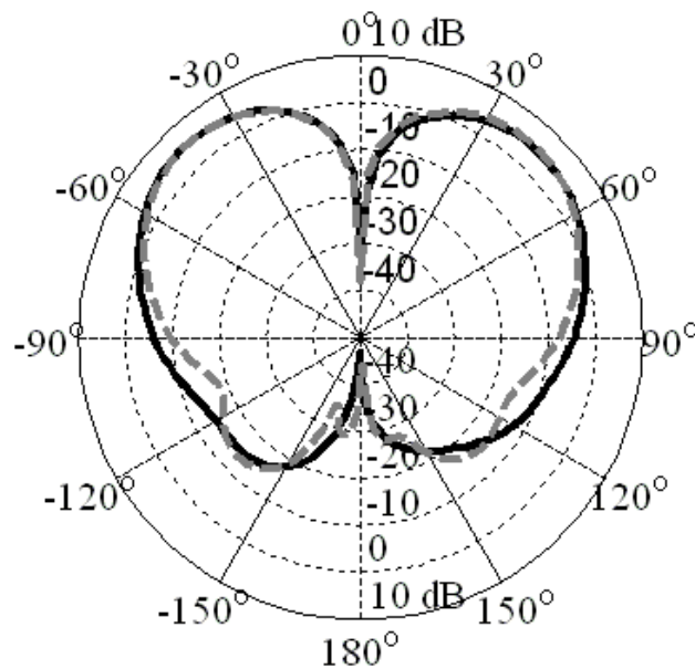
Figure 5. Measured radiation patterns in E-plane at 2.1 GHz of the carbon-fiber monopole antenna (grey dashed line) and of the copper counterpart (black solid line).
