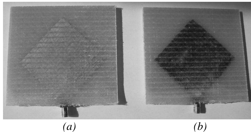
Figure 2. Pictures of the lozenge monopole antennas: (a) Copper radiating element embedded inside composite laminate (reference antenna); (b) Carbon-fiber radiating element (one ply) embedded inside composite laminate.
