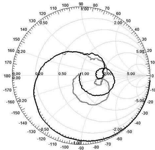
Figure 3. Measured input impedances (from 25 MHz to 3 GHz) of the carbon-fiber monopole antenna (grey dotted line) and of the copper counterpart (black solid line).
