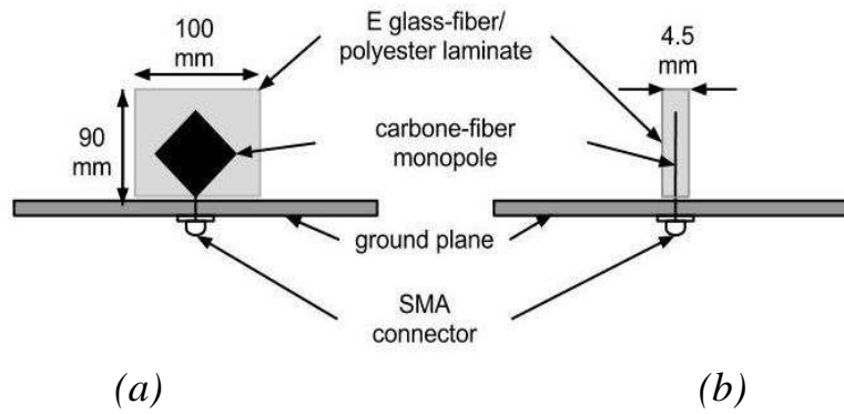
Figure 1. Lozenge monopole antenna: (a) front-view; (b) side-view.
