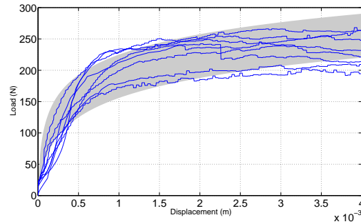
Figure 6: Comparison of the 8 experimental curves (eight solid lines) with confidence region calculated with the identified prior probability model (grey region) at 1500 s of thermal loading.
