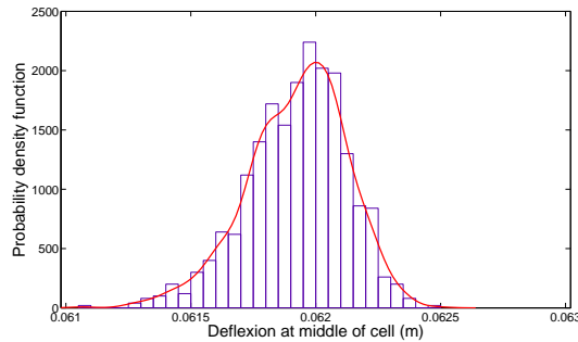
Figure 24: Thermal loading at 1200 s. Graph of the probability density function of the random deflection W at middle height of the large light partition wall.
