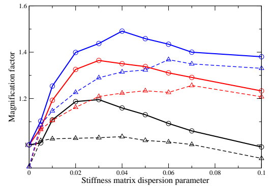
Fig. 9. Influence of the mistuning rate: graph such that P(B_\infty \leq B_p) = p . The solid curves with circles (and the dashed curves with triangles) are related to the tuned (and to the detuned) system. The lower, middle and upper curves correspond respectively to a probability level p = 0.50, 0.95 and 0.99 .
