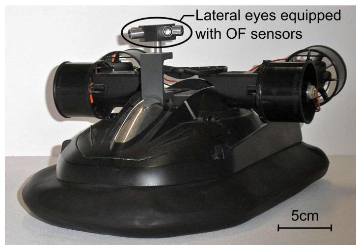
Figure 1. Sighted fully actuated hovercraft for testing the LORA III autopilot (Serres et al., 2008a).
