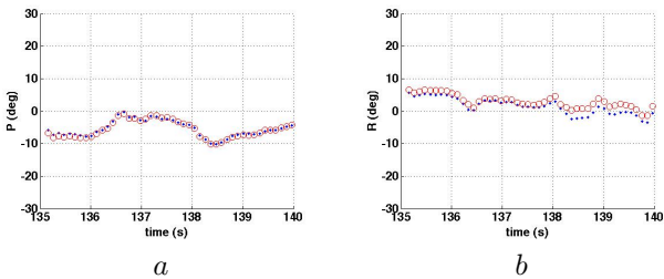
Fig. 10. Estimated P (a) and R (b) in the experiment. Blue dots indicate ground true values while red discs indicate the estimated values.
