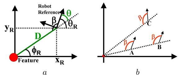
Fig. 2. A simple localization problem. The robot is equipped with odometry and bearing sensors able to evaluate the angle \beta . In b , the three initial robot configurations are compatible with the same initial observation ( \beta ).
