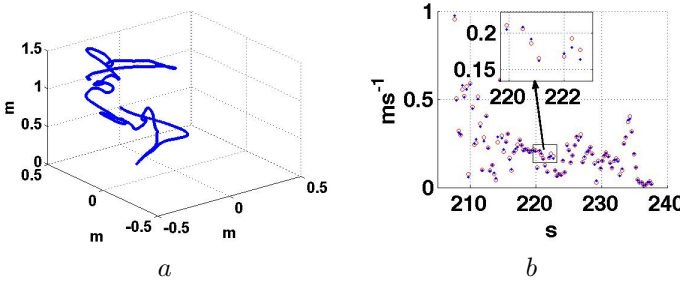
Fig. 10. In a : the trajectory (ground truth) in the 3D real data set during the time interval [200, 240]s. In b : the vehicle speed in the real 3D experiment. Blue dots are the ground truth and red disks the estimated values.
