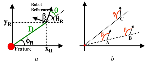
Fig. 2. A simple localization problem. The robot is equipped with odometry and bearing sensors able to evaluate the angle \beta . In b , the three initial robot configurations are compatible with the same initial observation ( \beta ).
