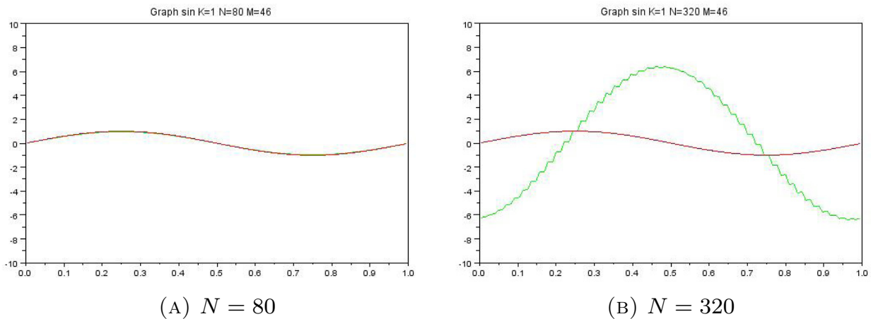
FIGURE A.1. Results for N = 80 (left) and N = 320 (right), using P_1 elements with M = 46 in both cases. Instability appears on the right figure.
