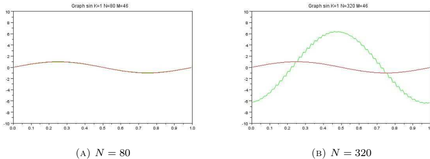
FIGURE 1. Results for N = 80 (left) and N = 320 (right), using P_1 elements with M = 46 in both cases. Instability appears on the right figure.
