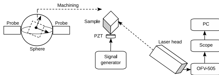
Figure 2: Whole experimental set-up from the identification of the material eigen directions on a sphere to the RUS measurements. The cubic sample cut from the sphere is excited by a PZT sending out a chirp signal. The induced vibrations are measured by the Laser Doppler Vibrometer.
