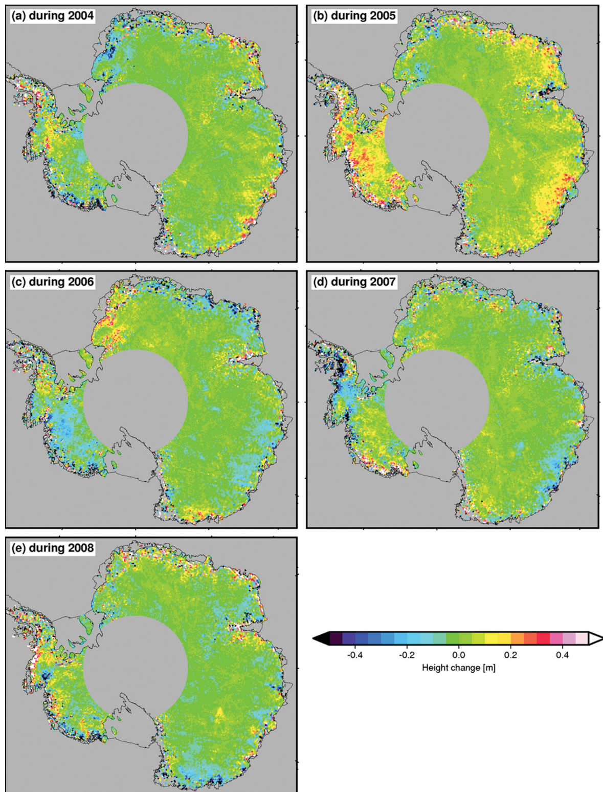
Figure 7. Year-to-year interannual variations of ENVISAT RA ice sheet thickness \Delta z(t) . The maps are analogous to Figs 6(a)–(e), but for the high-resolution grids. As in Fig. 6 the linear trend is not included.
