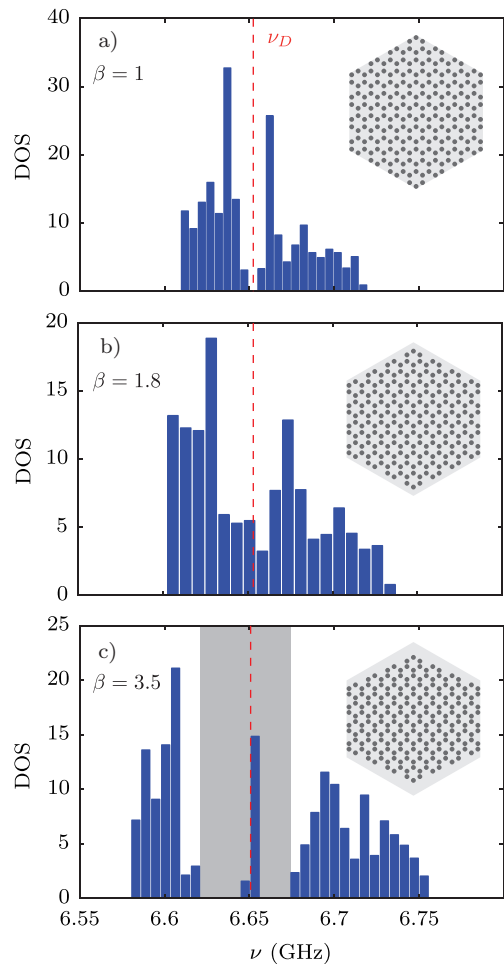
FIG. 2. Experimental DOS for a) the regular graphene ( \beta = 1 ), b) and c) anisotropic structures with \beta = 1.8 and \beta = 3.5 respectively. The dashed red lines indicate the Dirac frequency \nu_D . The gray zone shows the band gap with edge states at \nu_D .
