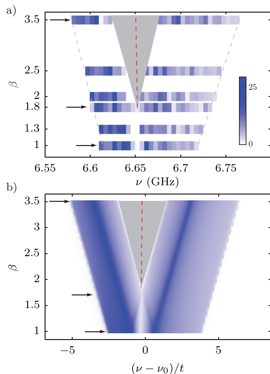
FIG. 3. a) Experimental DOS for \beta varying from 1 to 3.5. To remove edges states and highlight the band gap opening, the DOS have been averaged over bulk sites only. The gray zone shows the band gap opening and the red dashed line indicates the \nu_D position. The arrows at \beta = 1, 1.8 and 3.5 indicate the DOS plotted respectively in Fig. 2a, b and c, where the average was performed over all sites. b) Calculated DOS for \beta varying from 1 to 3.5 for an infinite system. The arrows at \beta = 1, 1.8 and 3.5 indicate the DOS plotted in Fig. 1b, d and f respectively.
