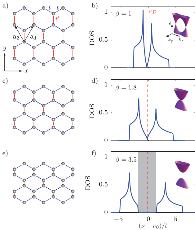
FIG. 1. Left panels: Schematics of the hexagonal lattices. \mathbf{a}_1 and \mathbf{a}_2 define the primitive cell of the Bravais lattice. t (blue intersite links) and t' (red ones, along y axis) correspond to the nearest-neighbor couplings. An anisotropy is introduced along the y axis. Right panels: Calculated density of states (DOS) for an infinite system with first, second and third nearest-neighbor couplings given in the text. The red dashed line is the Dirac frequency \nu_D = \nu_0 + 3t_2 . The insets show the corresponding dispersion relation. (a-b) Regular honeycomb lattice, \beta = 1 . The two Dirac points are distinguishable. (c-d) Compressed lattice at the topological transition, \beta = 1.8 . The Dirac points merge. (e-f) \beta = 3.5 , a band gap opens (gray zone).
