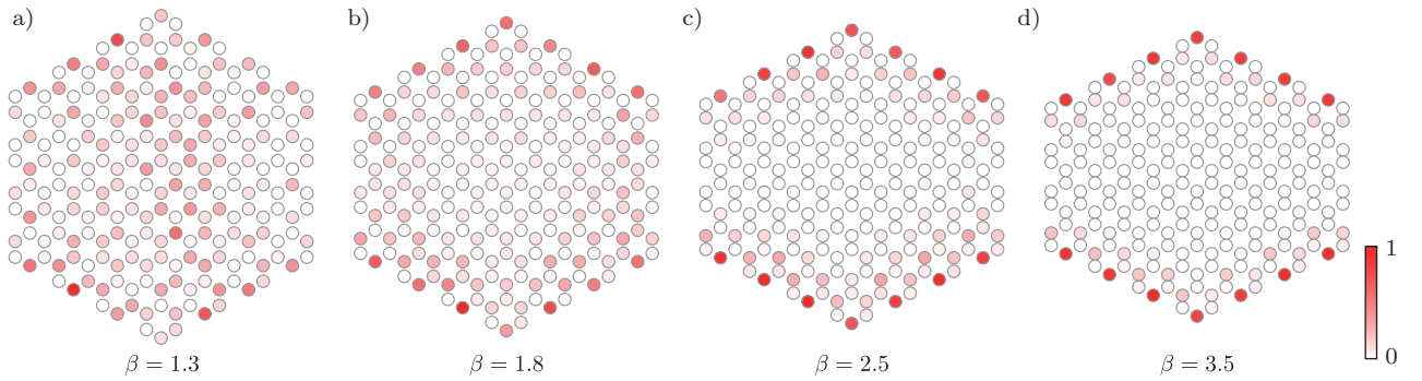
FIG. 4. Experimental wave function distributions at the Dirac frequency \nu_D (red dashed line in Fig. 3) for \beta ranging from 1.3 to 3.5.
