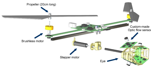
Fig. 2. Schematic CAD of the BeeRotor robot. It is composed of a main electronic board called the body, which carries most of the sensors and actuators, performs all the data processing and controls the rotorcraft. The pantographic arm to which this board is connected simply provides the aircraft with its power requirements. The main electronic board is composed of two elongated arms connected to two propellers controlled by Brushless outrunner motors. The robot’s eye, which is set apart from the main board to prevent the visual field from being occluded by the propellers, is composed of 4 custom-made optic flow sensors based on an off-the-shelf photosensor array combined with the “time of travel” scheme. The eye can rotate independently from the body of the aircraft thanks to the presence of a stepper motor.
