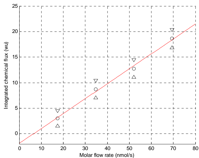
Figure 13-c: Integrated chemical heat source in the channel at different flow rates.
