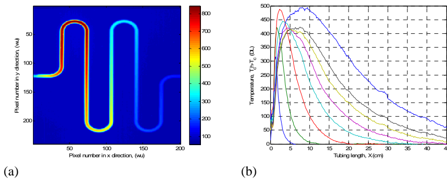
Figure 10. a) IR image of chip corresponding to T_{ch} = T-T_0 at Q_a=Q_b=60 \text{ mL.h}^{-1} and T_c=10^\circ\text{C} ; b) temperature due to the chemical reaction ( T_{ch}-T_c ) versus tubing length for various flow rates: 2, 4, 10, 20, 30, 40, 50, 60 \text{mL.h}^{-1}
