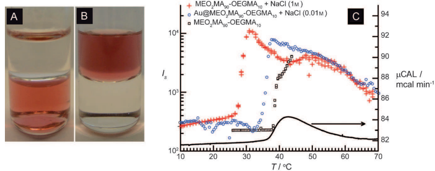
Figure 1. A) Au@MEO 2 MA 90 -co-OEGMA 10 NPs well dispersed in water (at room temperature) with a clear toluene phase on top and B) NP transfer to toluene upon adding salt under stirring. The NP concentration in water is 50 mg L -1 . C) Temperature-dependent light scattered intensity profiles of MEO 2 MA 90 -co-OEGMA 10 copolymer (10 g L -1 ) in pure water (squares) and 1 M NaCl solution (crosses) and Au@MEO 2 MA 90 -co-OEGMA 10 NPs with 10 mM NaCl solution (50 mg L -1 , circles). The black curve shows microcalorimetry raw data for the polymer in water. The heating rate ( \delta T/\delta t ) is 6 °C h -1 .
