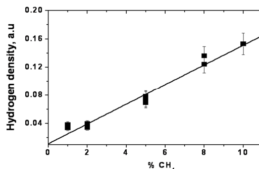
Fig. 1: Evolution of hydrogen atom densities as a function of % CH 4 .
