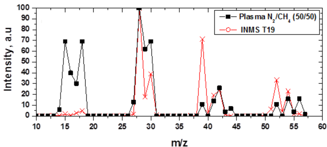
Fig. 2: Qualitative comparison of positive ion mass spectra observed in a N_2 - CH_4 RF plasma [6] and in Titan's ionosphere (INMS T19), in arbitrary units and normalized at m/z 28.
