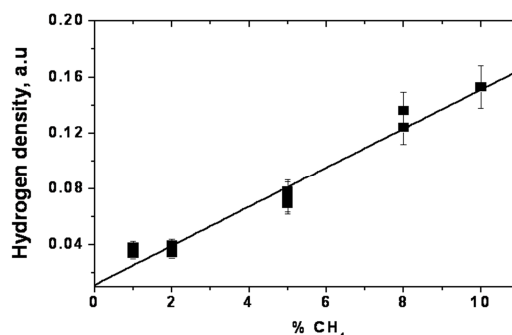
Fig. 1: Evolution of hydrogen atom densities as a function of % CH 4 .
