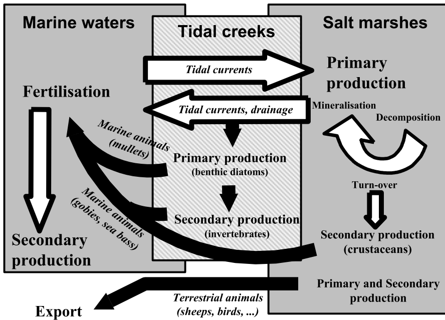
Figure 1. Exchanges of organic matter between saltmarsh and coastal marine water by abiotic and biotic vectors in the bay of Mont Saint-Michel.
