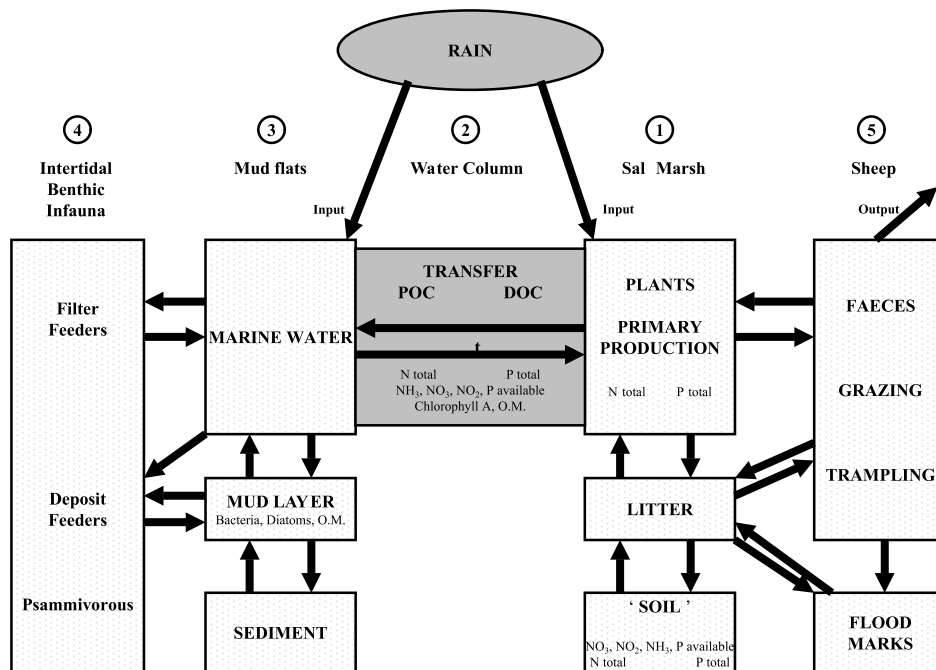
Figure 2. Schematic presentation of the compartment model used to study the saltmarsh functioning and exchanges between salt marsh and coastal marine systems. Example of the bay of Mont Saint-Michel (Lefeuve et al., 1994).
