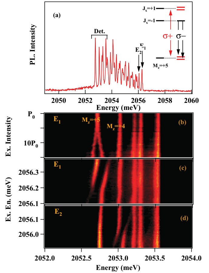
FIG. 5. (Color online) (a) Nonresonant PL of X -2Mn in QD1. The inset illustrates the effect of a \sigma+ resonant laser field on M_z = +5 ( E_1 ). (b) PL intensity map of the X -2Mn versus the power of the control laser in resonance with E_1 . (c, d) PL maps of the X -2Mn when the control laser energy is tuned around E_1 (c) and E_2 (d).
