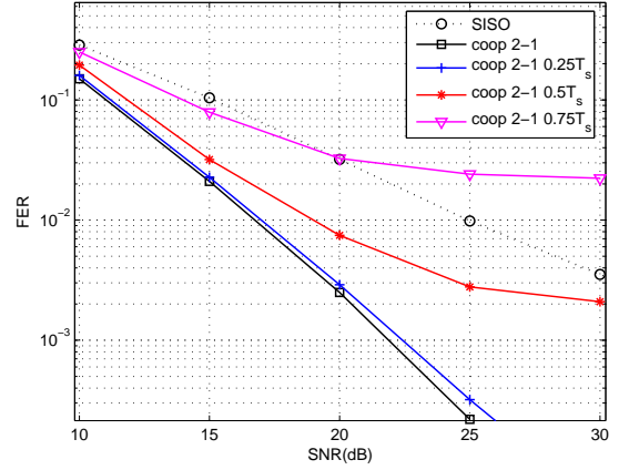
Fig. 5. Effect of the transmission synchronization error on the performance of cooperative MISO systems with two transmit nodes N = 2 , Alamouti STBC over a Rayleigh fading channel.
