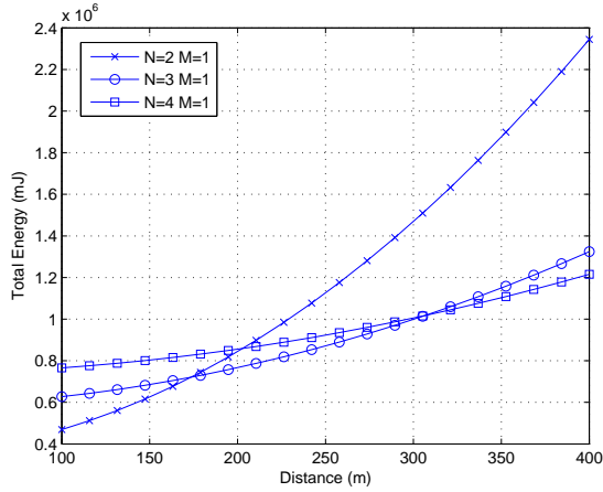
Fig. 14. Energy Consumption of cooperative MISO technique with two, three and four transmission nodes, power path-loss factor K = 2 , FER = 10^{-3} , Rayleigh fading channel.
