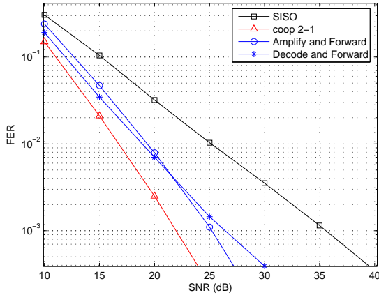
Fig. 4. FER of relay technique vs. cooperative MISO technique with two transmission nodes, non-coded QPSK modulation over a Rayleigh channel, 120 bits/frame, source-relay distance d_1 = d/3 , and power path-loss factor K=2 .
