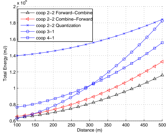
Fig. 16. Total energy consumption of cooperative MIMO with different reception techniques vs. cooperative MISO, \Delta T_{syn} = 0.25T_s , FER = 10^{-3} requirement, Rayleigh fading channel with power path-loss factor K = 2 .
