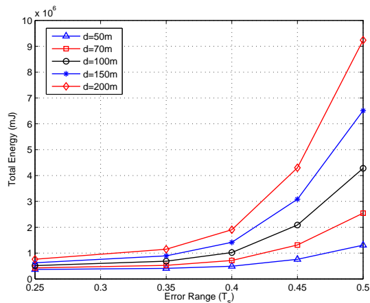
Fig. 19. Energy Consumption of cooperative MISO technique in function of transmission synchronization error range, two transmission nodes, error rate FER = 10^{-3} requirement, Rayleigh fading channel with the power path-loss factor K = 2
