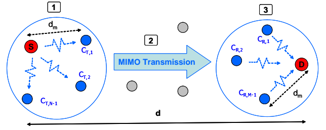
Fig. 3. Cooperative MIMO transmission scheme from S to D with N cooperative transmission nodes ( S, C_{T,1}, C_{T,2}, \dots, C_{T,N-1} ) and M cooperative reception nodes ( D, C_{R,1}, C_{R,2}, \dots, C_{R,M-1} ).
