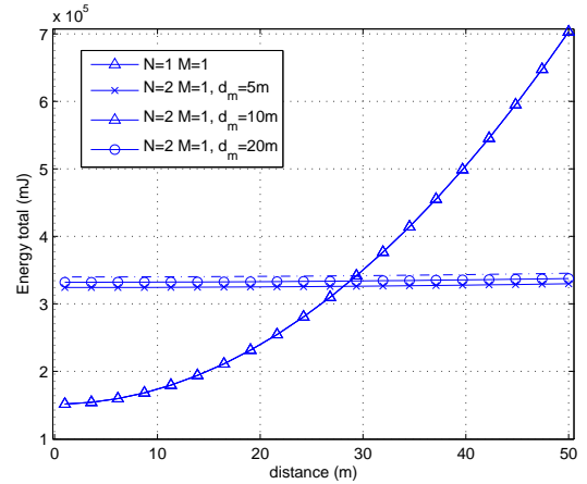
Fig. 15. Energy consumption of the cooperative MISO 2 – 1 with different cooperative transmission distances d_m = 5, 10 and 20\text{m} , FER = 10^{-3} requirement, Rayleigh block fading channel with power path-loss factor K = 2 .
