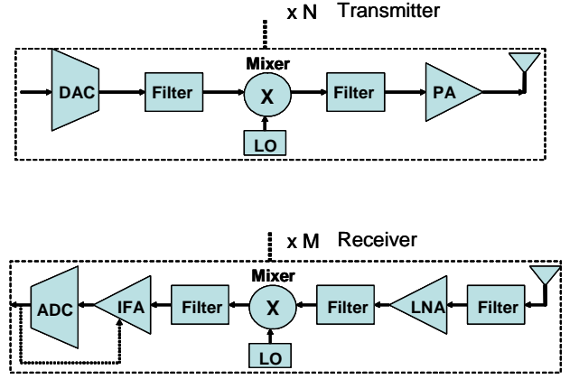
Fig. 12. Transmitter and receiver blocks with N transmit and M receive antennas.
