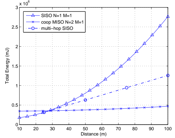
Fig. 13. Energy Consumption of SISO vs. cooperative MISO technique with two transmission nodes, power path-loss factor K = 2 , FER = 10^{-3} , Rayleigh fading channel.
