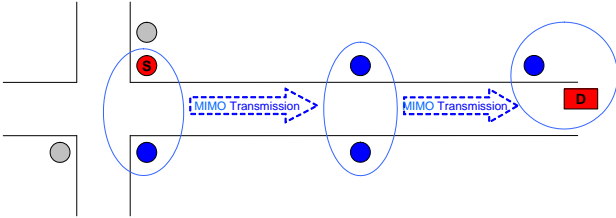
Fig. 11. Multi-hop cooperative MIMO transmission between infrastructure and vehicle
