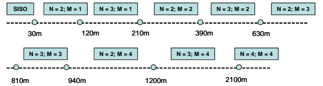
Fig. 17. Optimal N - M transmit and receive antennas set selection as a function of transmission distance, \Delta T_{syn} = 0.25T_s , FER = 10^{-3} requirement, Rayleigh fading channel with power path-loss factor K = 2 .
