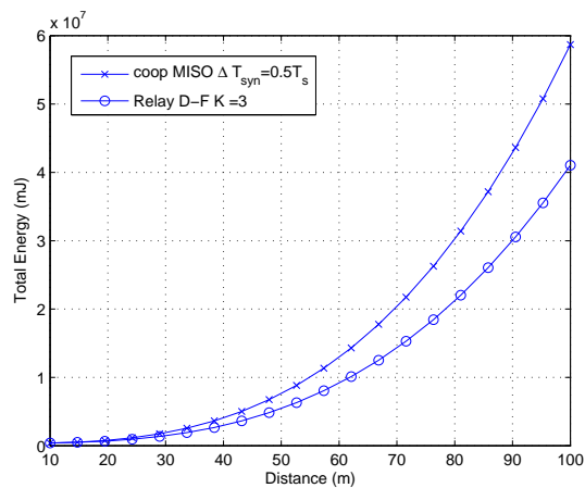
Fig. 20. Energy consumption of relay technique vs. cooperative MISO technique with two transmission nodes N = 2 , power path-loss factor K = 3 , error rate FER = 10^{-2} , transmission synchronization error range \Delta T_{syn} = 0.5T_s and source-relay distance d_1 = d/3 .
