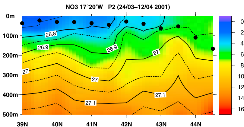
Figure 2. Section of isopycnal depths (contours for \sigma surfaces) and nitrate (color scale in mMol kg -1 ) along 17°20'W during P2. The actual mixed layer depths (0.02 density jump criterion) are indicated by dots.
