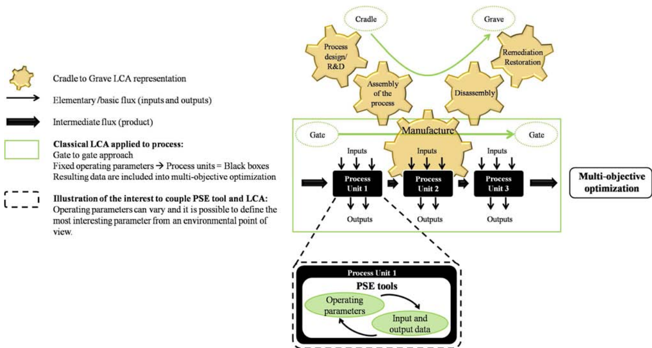
Figure 3. Illustration of PSE tool integration into LCA methodology for process
