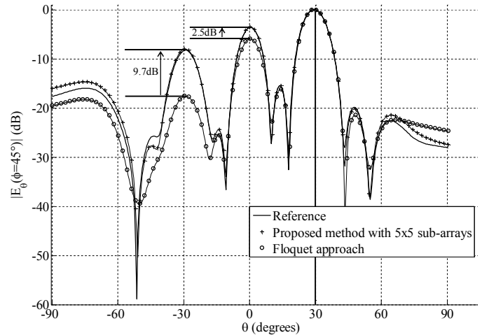
Fig. 10. Analysis of a 10x10 reflectarray with the proposed method with 5x5 sub-arrays, the Floquet approach and the global simulation.
