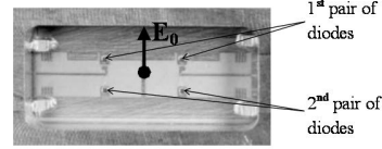
Fig. 4. Reflectarray phase shifting cell.
