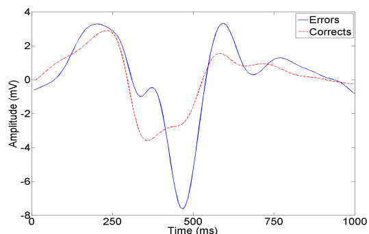
Fig. 2: Mean potential averaged over 21 subjects at electrode FCz.
