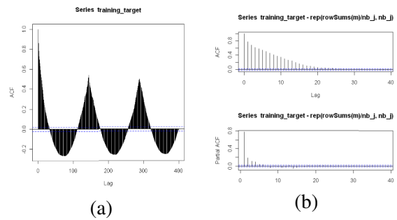
Figure 7: Autocorrelation diagrams for the PEMS data.
