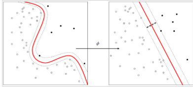
Figure 5: Illustration of the kernel trick (source: Wikipedia).
