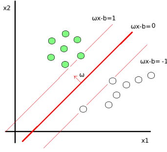
Figure 4: SVM as a binary classifier.
