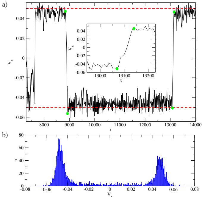
FIG. 8: (color online) (a) Center of mass velocity fluctuations in steady state for V=0.05 in a system with L_x=20 and L_y=20 . The dashed red lines represent the velocity of the top and bottom walls. The transition time (magnified in the inset) is measured at both ends of direct transitions from one wall to the other, between the round dots. (b) Histogram of center of mass velocities.
