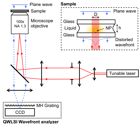
FIG. 1. Experimental configuration used to perform quantitative absorption spectroscopy measurements. The inset illustrates the wavefront distortion thermally induced by the heated NP.
