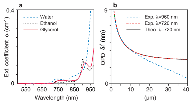
FIG. 4. a) Absorption spectra of various liquids. b) Radial profile of the OPD distribution around a single gold NP at \lambda_0 = 720 nm and \lambda_0 = 960 nm ( D = 6.2 \mu\text{m} et h = 7 \mu\text{m} ). In the second case, the heating of the liquid is responsible of an abnormal linear slope at large distances.
