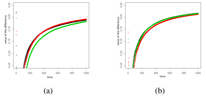
Fig. 1. Difference between the best achievable cumulative regret and the one obtained with the internal regret minimization algorithm in (a) and with the external regret minimization algorithm in (b) under full competition.
