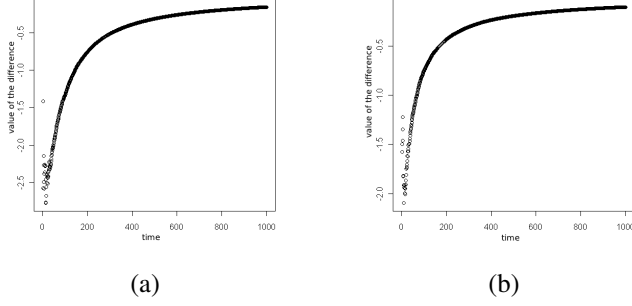
Fig. 2. Difference between the best achievable cumulative regret and the one obtained with the internal regret minimization algorithm in (a) and with the external regret minimization algorithm in (b) for the grand coalition of providers.
