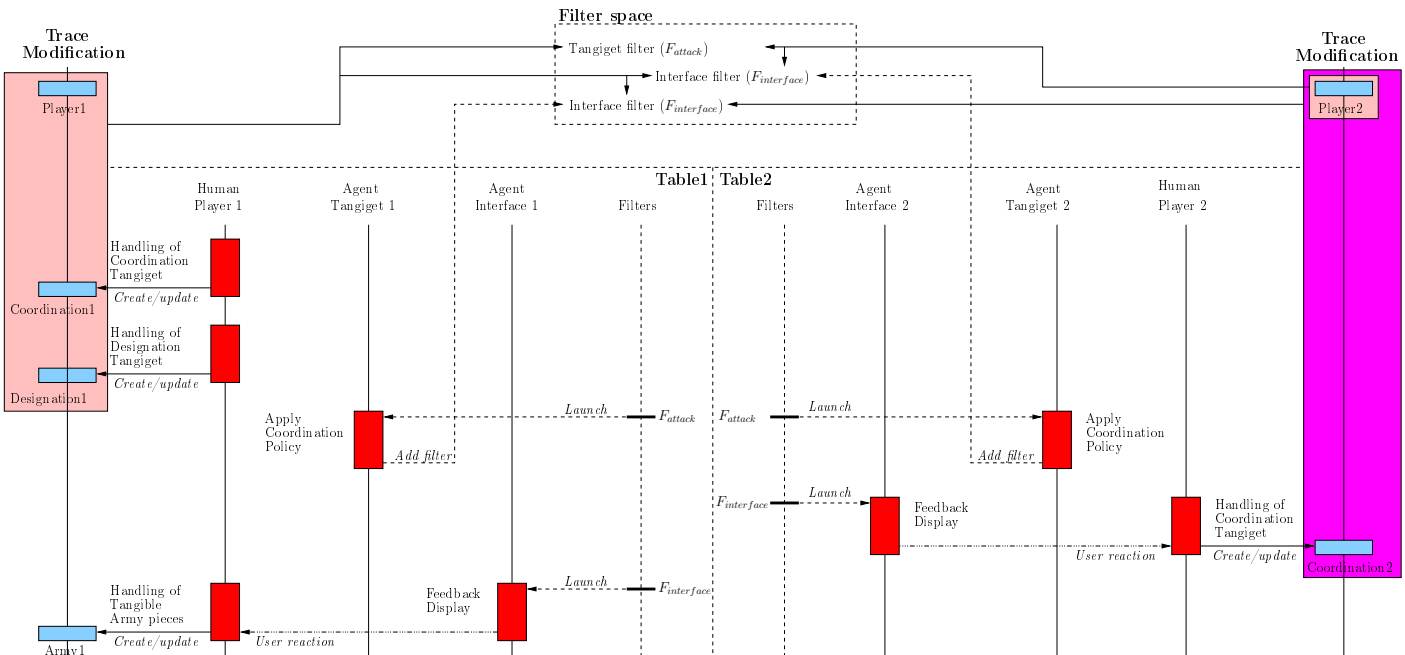
Fig. 4 Interleaving of tanginet, filter and agent activity to ensure activity coordination in a specific phase of the RISK game.
