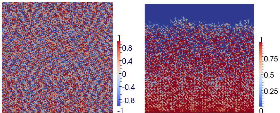
Figure 7: Cellwise constant parameter \gamma for the rocktype on the triangular mesh with 7297 nodes (left) and discrete oil saturation s_{\mathcal{D}} computed with the upwind scheme for kr_{\min} = 0 with this random capillary pressure.
