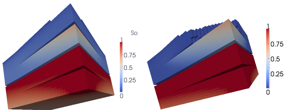
Figure 10: Plot of the oil saturation at final time for s_D > 0.05 computed with the upwind scheme and kr_{\min} = 10^{-3} (left) and kr_{\min} = 10^{-4} (right).
