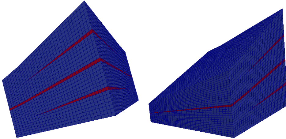
Figure 8: Hexahedral mesh (with degeneracies of some hexahedra due to erosion) of the domain with the three barriers in red (rocktype \beta in the red barriers and \alpha outside the barriers).
