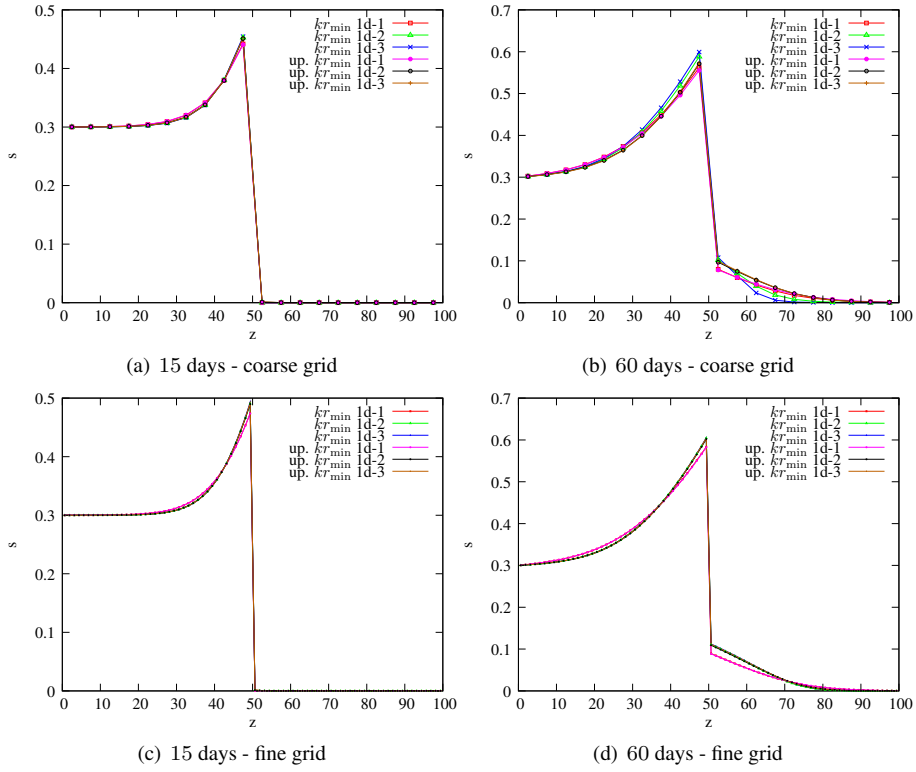
Figure 1: Oil saturation along the z axis after 15 and 60 days of simulation obtained for the centered scheme and the upwind scheme denoted by “up”.
