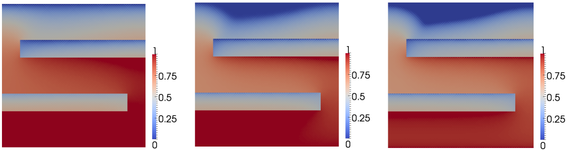
Figure 6: Comparison of the discrete oil saturation s_{\mathcal{D}} at final time on the uniform Cartesian 64 \times 64 , mesh computed with the upwind scheme and different values of k_{\min} = 10^{-1}, 10^{-2}, 10^{-3} from left to right.
