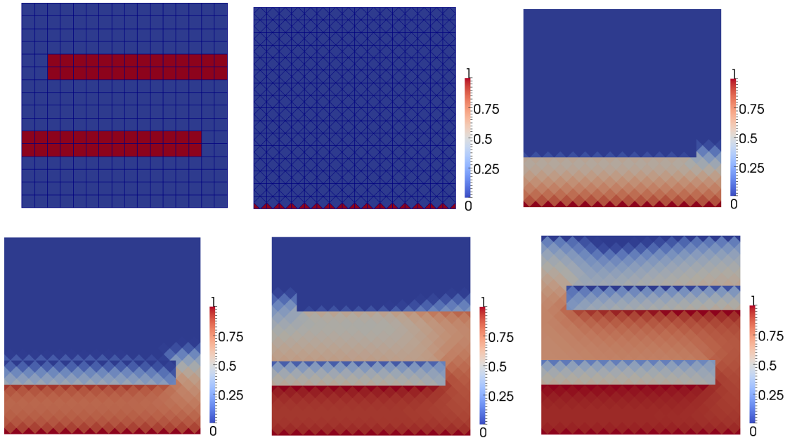
Figure 3: Test case with two barriers with rocktype \beta in the barrier and rocktype \alpha outside.
