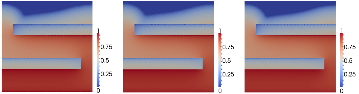
Figure 5: Comparison of the discrete oil saturation s_{\mathcal{D}} at final time computed with the upwind scheme and kr_{\min} = 0 on the uniform Cartesian 64 \times 64 , grid, a random quadrangular 64 \times 64 mesh, and a triangular mesh with 7297 nodes.
