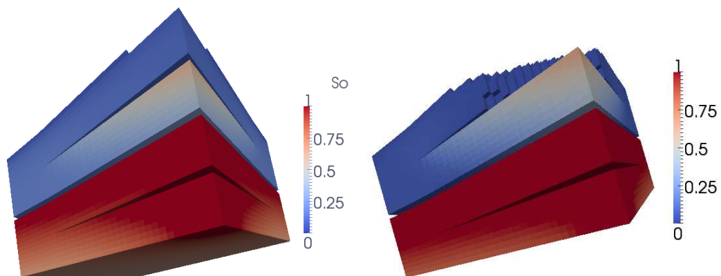
Fig. 10 Plot of the oil saturation at final time for s_D > 0.05 computed with the upwind scheme and kr_{\min} = 10^{-3} (left) and kr_{\min} = 10^{-4} (right).
