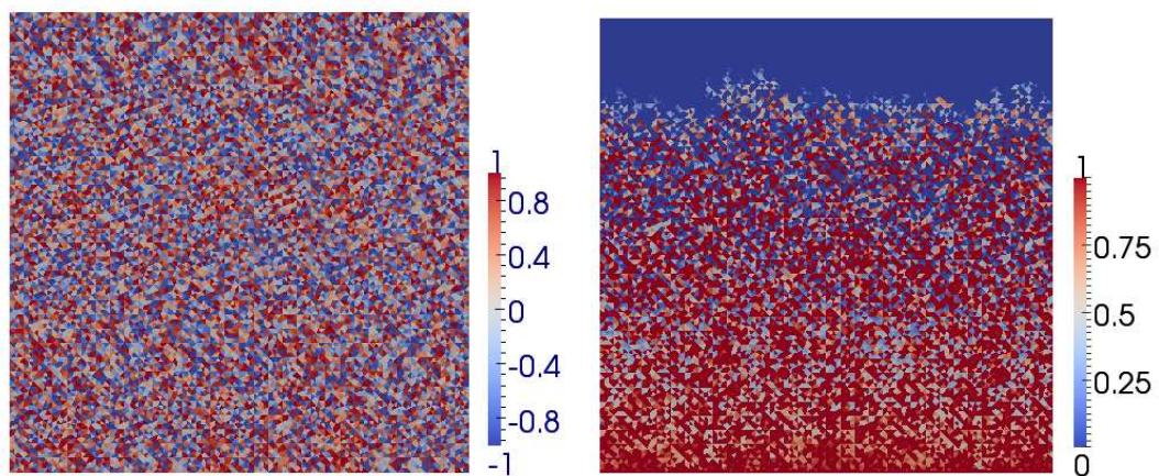
Fig. 7 Cellwise constant parameter \gamma for the rocktype on the triangular mesh with 7297 nodes (left) and discrete oil saturation s_{\mathcal{D}} computed with the upwind scheme for kr_{\min} = 0 with this random capillary pressure.
