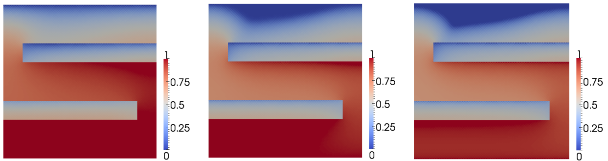
Fig. 6 Comparison of the discrete oil saturation s_{\mathcal{D}} at final time on the uniform Cartesian 64 \times 64 , mesh computed with the upwind scheme and different values of k_{\min} = 10^{-1}, 10^{-2}, 10^{-3} from left to right.
