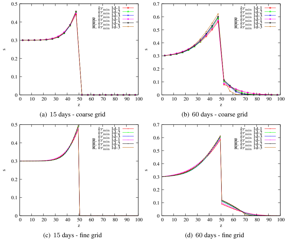
Fig. 2 Oil saturation along the z axis after 15 and 60 days of simulation obtained for the centered scheme and Richards denoted by “R.”.
