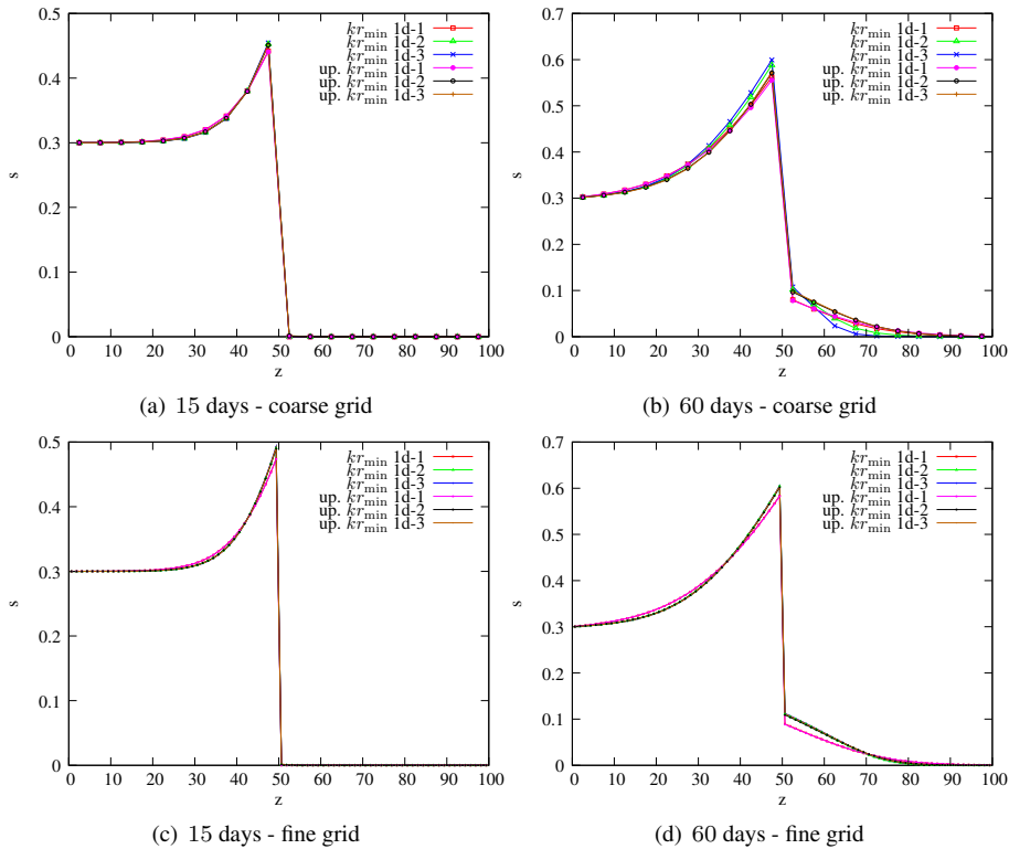
Fig. 1 Oil saturation along the z axis after 15 and 60 days of simulation obtained for the centered scheme and the upwind scheme denoted by “up”.
