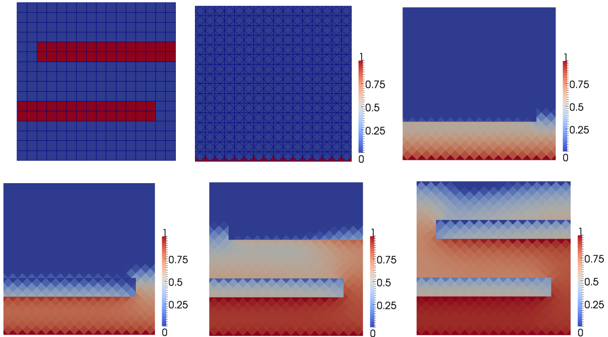
Fig. 4 Cartesian mesh and discrete oil saturation s_{\mathcal{D}} at successive times computed with the upwind scheme and kr_{\min} = 0 on the 16 \times 16 uniform Cartesian grid.
