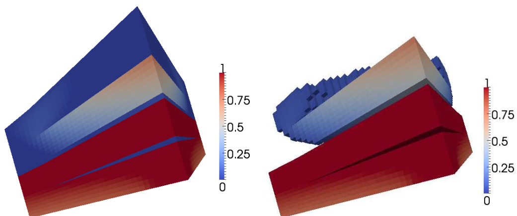
Fig. 9 Discrete oil saturation s_D at final time computed with the upwind scheme and kr_{\min} = 0 . On the right side plot of the oil saturation at final time for s_D > 0.05
