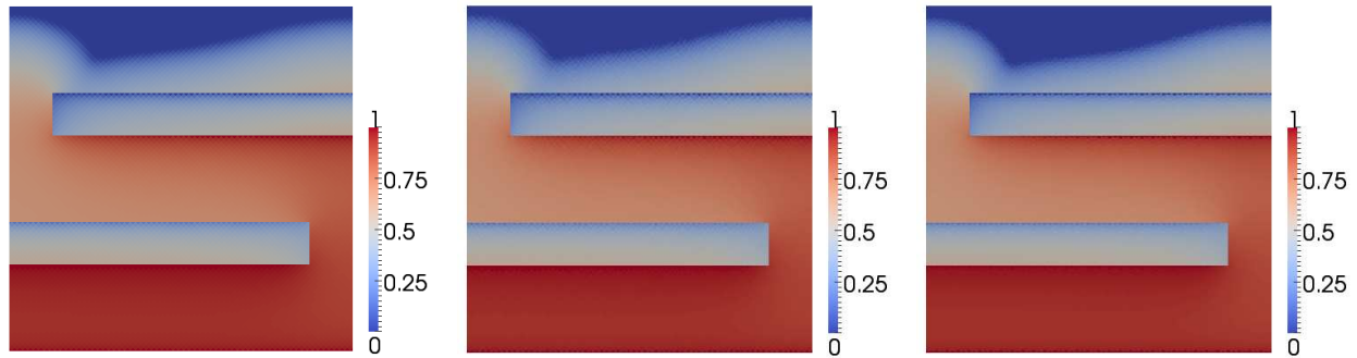
Fig. 5 Comparison of the discrete oil saturation s_{\mathcal{D}} at final time computed with the upwind scheme and kr_{\min} = 0 on the uniform Cartesian 64 \times 64 , grid, a random quadrangular 64 \times 64 mesh, and a triangular mesh with 7297 nodes.
