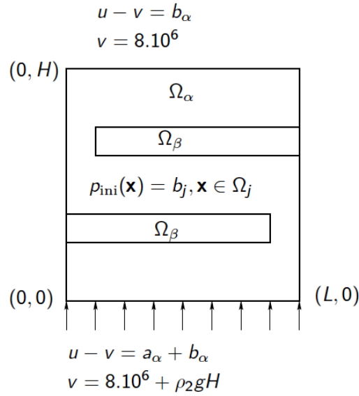
Fig. 3 Test case with two barriers with rocktype \beta in the barrier and rocktype \alpha outside.
