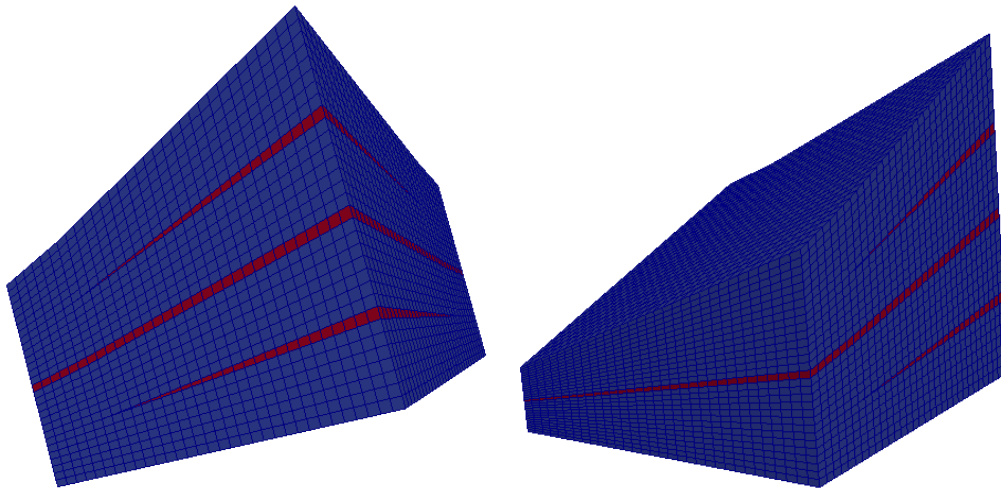
Fig. 8 Hexahedral mesh (with degeneracies of some hexahedra due to erosion) of the domain with the three barriers in red (rocktype \beta in the red barriers and \alpha outside the barriers).
