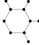
Figure 3: The consecutive broken sun CBSun_{6,4}
