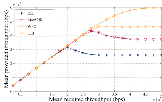
Fig. 11. Relay efficiency.
