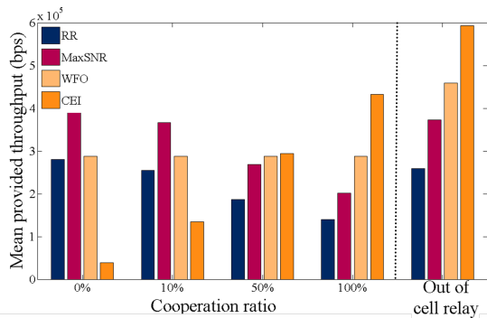
Fig. 12. Provided throughput function of cooperation ratio in overloaded system.
