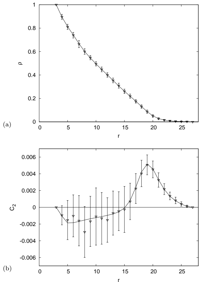
FIG. 7. Profile of 7(a) the density and 7(b) the connected correlation at time t = 450 for the gap junctional model on a radial geometry with r_{src} = 3 and r_{snk} = 27 . The lines show the results of 3 \cdot 10^6 averaged independent stochastic simulations at time t with same initial conditions and parameter p=1 . The dots and the bars represent the average and the error for only 10^3 stochastic simulations.
