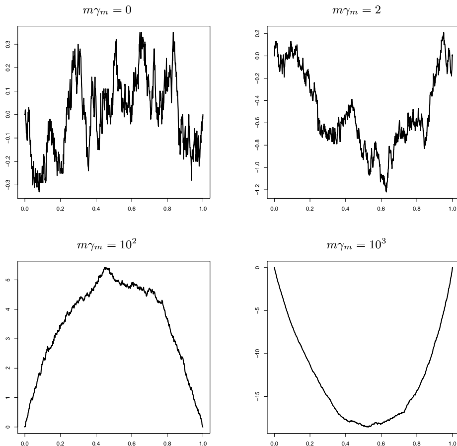
FIG 1. Plot of t \mapsto m^{1/2}(\widehat{\mathbb{F}}_m(t) - t) for some observed Y(\omega) . These realizations have been generated in the equi-correlated model \Gamma_{i,j}^{(m)} = \rho_m , i \neq j (see (14)) and for m = 10^4 .
