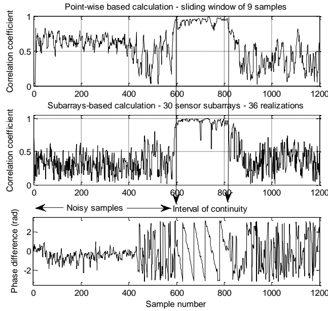
Fig. 5. Estimation of the correlation coefficient (after beam forming at 55°) based on the point-wise approach (18) (upper plot) compared with the estimation based on sliding pairs of sub-arrays, each one providing a realization of signals S_1 and S_2 . The result is the generation of an interval of continuity as described in Section IV-A. Parameters: f= 300 kHz, z= 23 m
