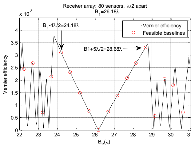
Fig. 9. For a given baseline B_1 , the second baseline length can be determined by analyzing the Vernier efficiency (solid line). Applied to multibeam echosounders, only some array configurations are feasible according to the number of sensors composing the sub-arrays (in circles).
